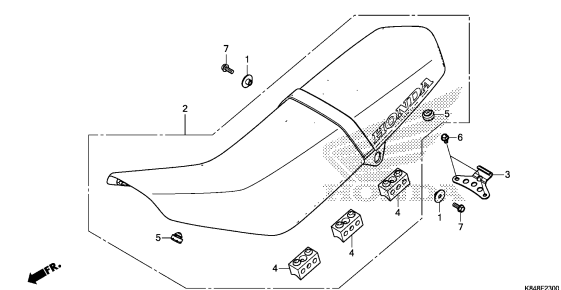
SEAT
