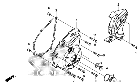
LEFT CRANKCASE COVER
