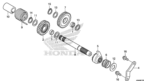
KICK STARTER SPINDLE
