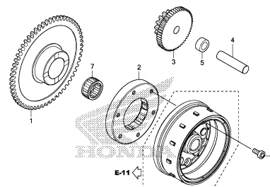
STARTING CLUTCH
