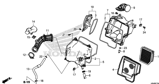
AIR CLEANER
