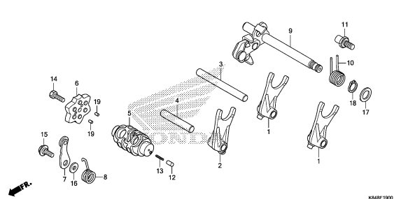
GEARSHIFT DRUM
